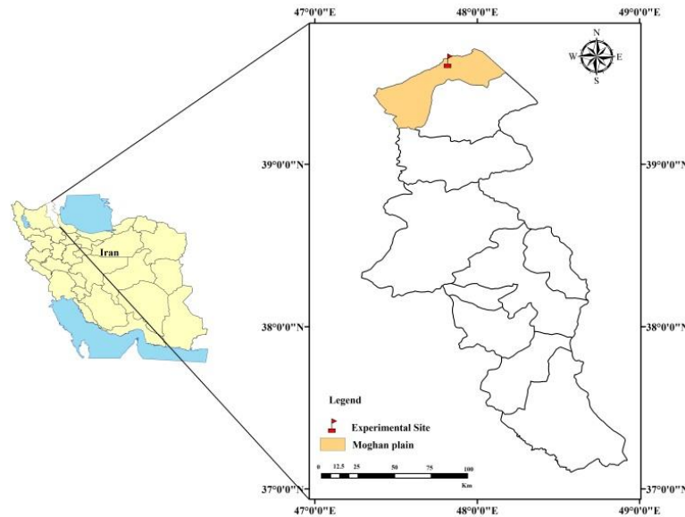
Fig. 1 Map of Iran showing the location of the experimental site
