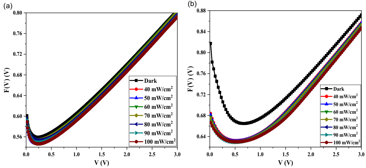
Figure 5. The variations of the F(V) – V curves of the a) MS- and b) MPS-type PDs at in the dark and under different illumination intensities.
