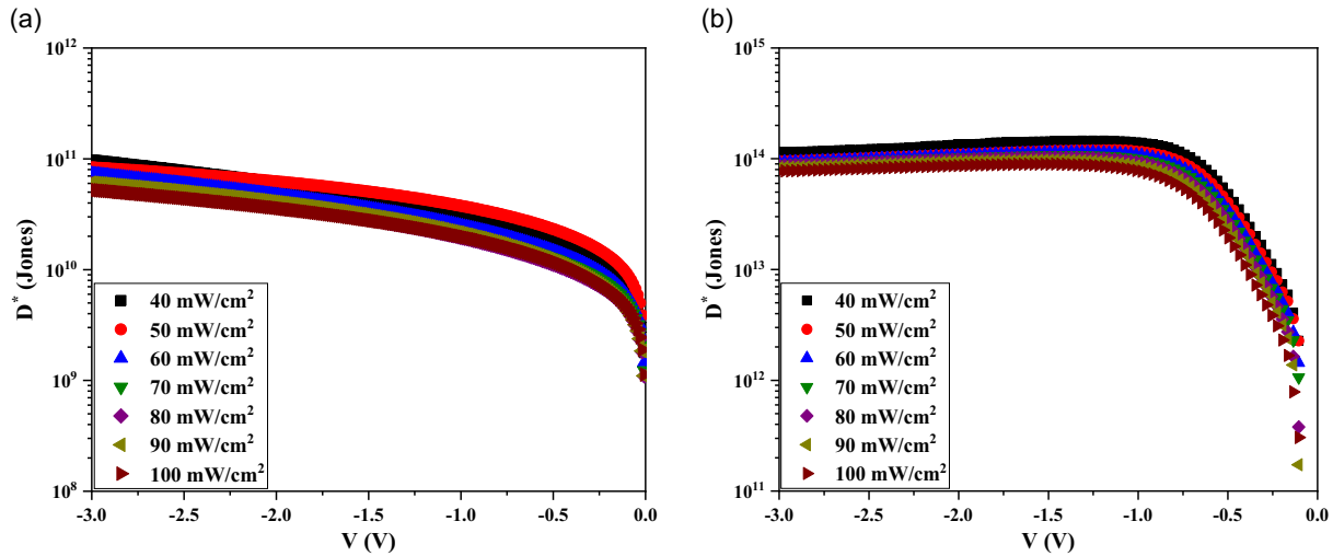
Figure 12. The changes of D - V graphs of the a) MS- and b) MPS-type PDs illuminated by different intensities.
