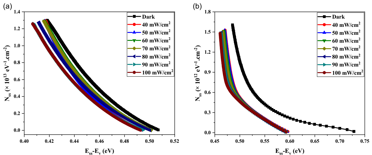
Figure 6. Variations of the interface states density in terms of energy for the a) MS and b) MPS PDs in the dark and under illumination.
