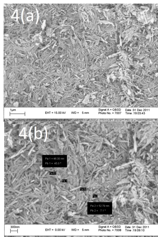
Fig. 4(a) and (b). SEM images of \alpha -Fe 2 O 3 nanostructures prepared by ultrasound-assisted method at different magnifications.
