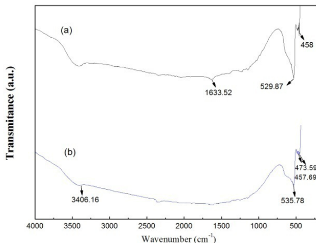
Fig. 5. FT-IR Transmittance spectrum of the prepared samples before thermal annealing (FeO(OH))(a) and after thermal annealing at 450 °C (sample \alpha -Fe 2 O 3 )(b).
