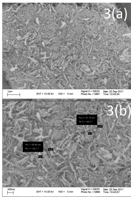
Fig. 3(a) and (b). SEM images of FeO(OH) nanostructures prepared by ultrasound-assisted method at different magnifications.
