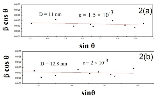
Fig. 2(a). plot of \beta \cos \theta vs. \sin \theta for FeO(OH) and 2(b) for \alpha -Fe 2 O 3 nanostructures prepared by ultrasound-assisted method.
