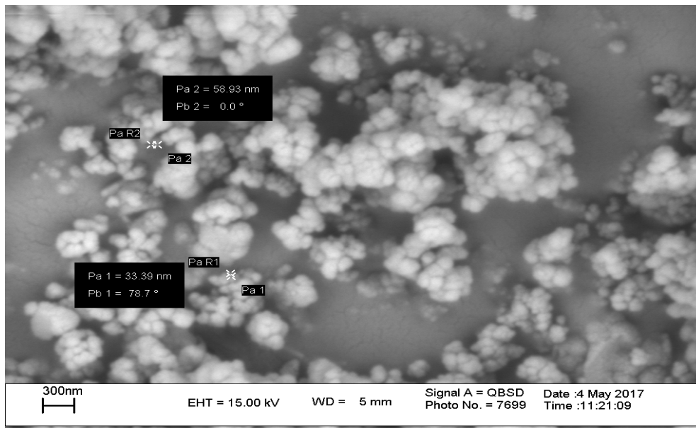
Figure 1. Scanning electron microscope micrograph of potassium silicate nanoparticles
