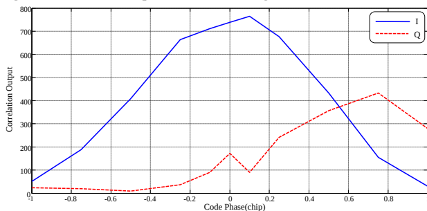
Fig. 8 Correlation output of spoofed signal (case 1).
